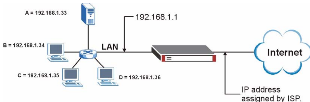
Figure 205 Multiple Servers Behind NAT Example
