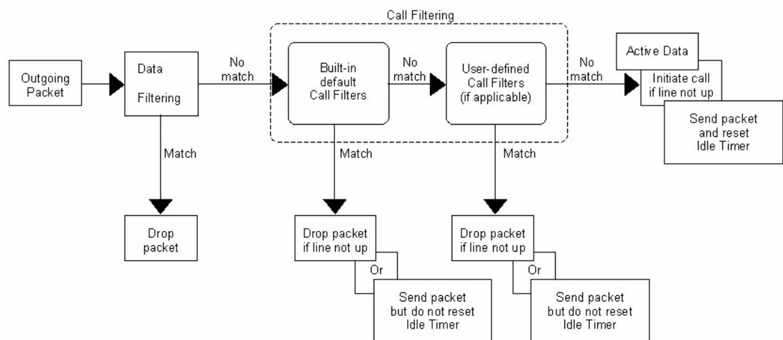
Figure 347 Outgoing Packet Filtering Process
