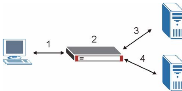
Figure 141 Content Filtering Lookup Procedure
