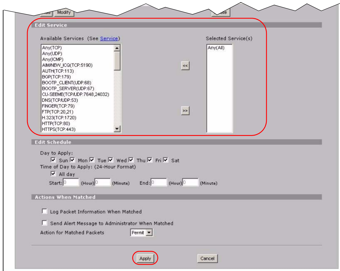
Figure 65 Tutorial Example: Firewall Rule: WAN to LAN Service Edit for Mail Server
