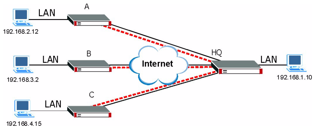
Figure 176 Telecommuters Using Unique VPN Rules Example
