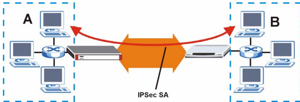
Figure 462 Managing the Bandwidth of an IPsec SA
