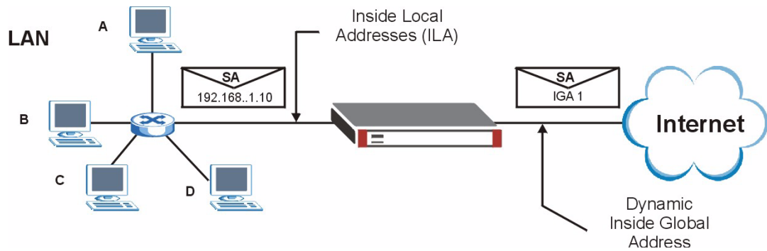
Figure 333 Menu 4: Internet Access &amp; NAT Example
