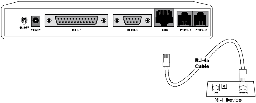
Figure 2 -3 Hooking Up an NT-1 Device
