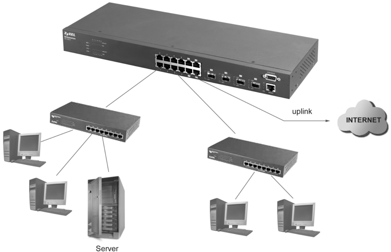
Figure 1-2 Bridging Application
