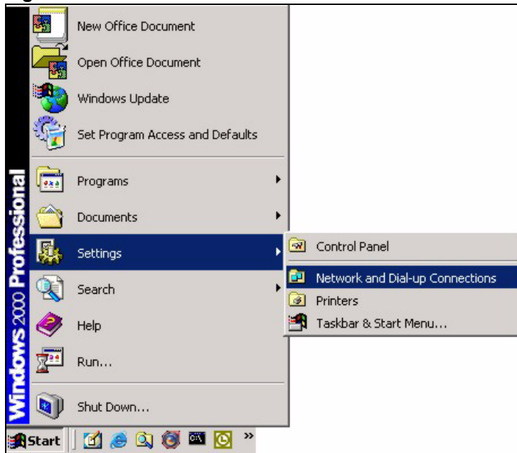
Figure 45 Windows 2000: Start
