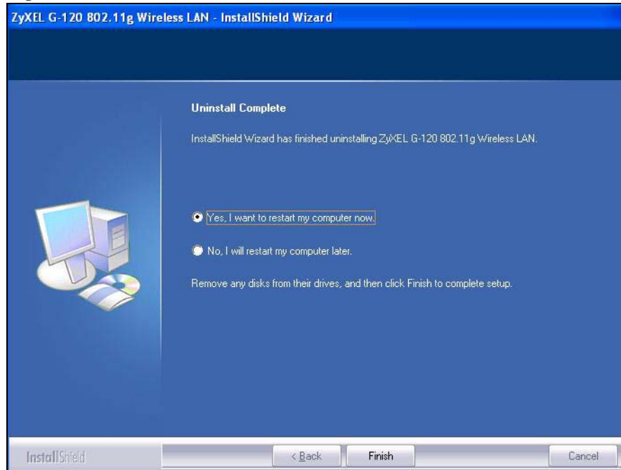
Figure 44 Uninstall: Finish
