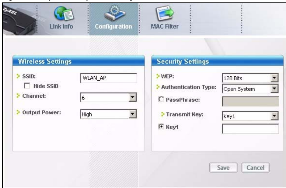
Figure 19 ZyXEL Utility: AP: Configuration
