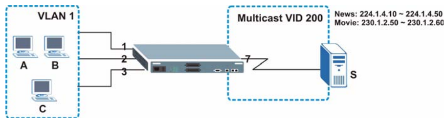
Figure 68 MVR Configuration Example
