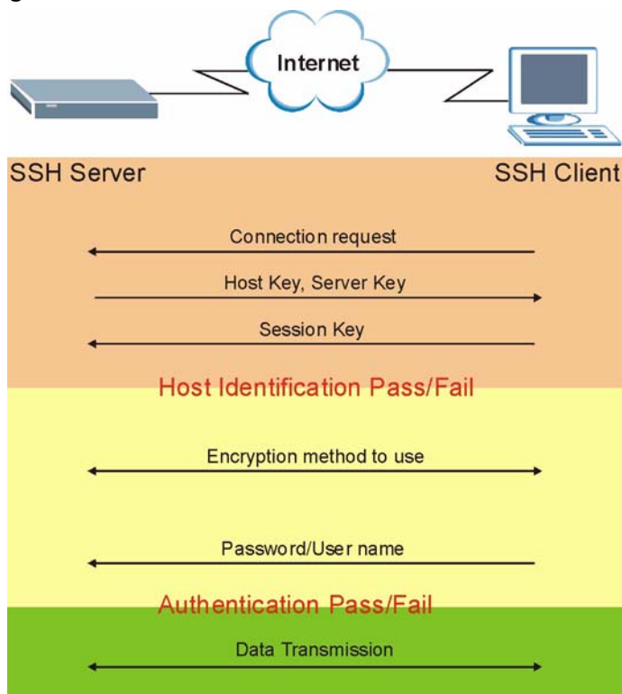
Figure 87 How SSH Works
