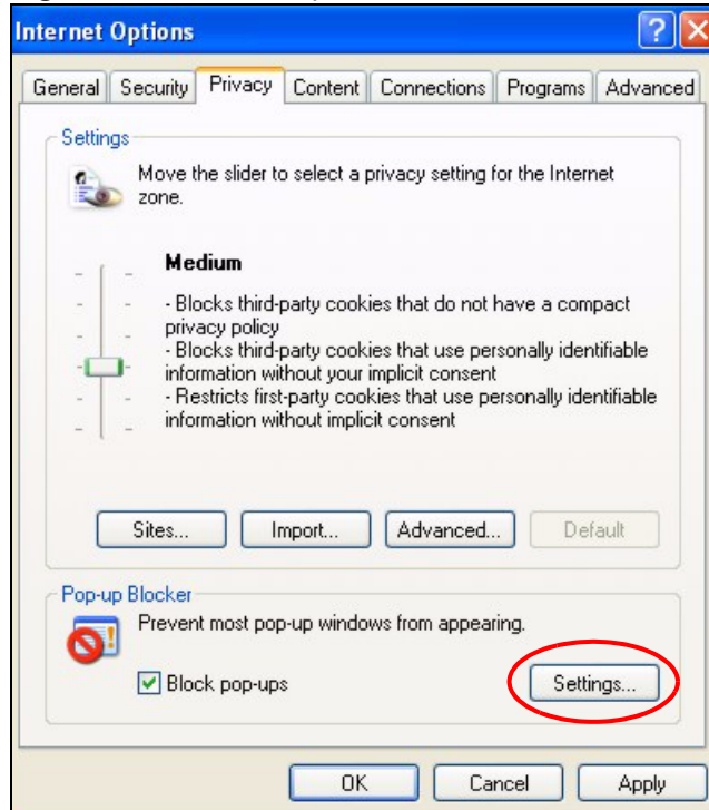
Figure 111 Internet Options
