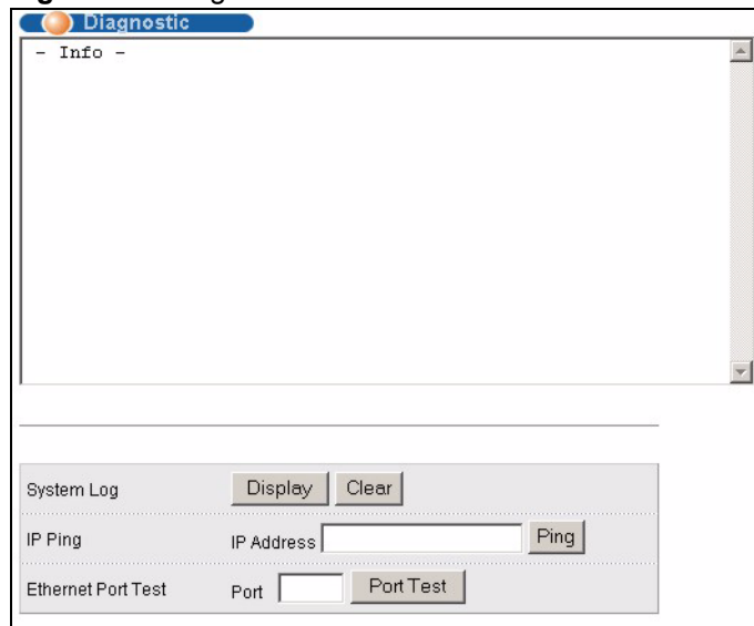
Figure 96 Diagnostic
