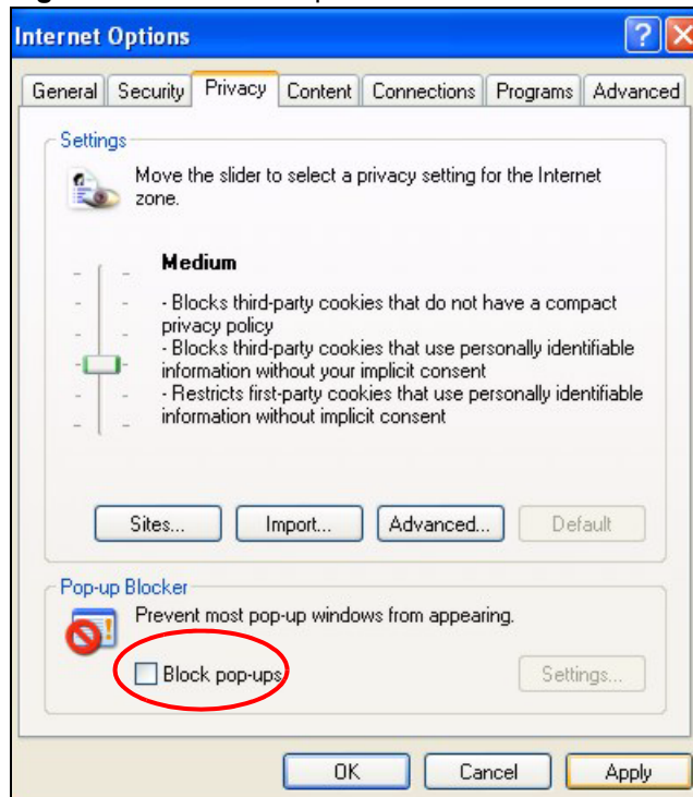
Figure 110 Internet Options
