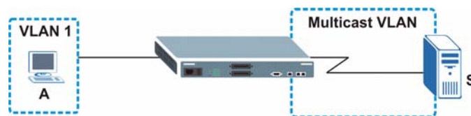
Figure 65 MVR Multicast Television Example
