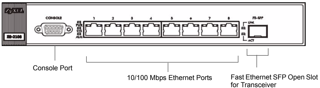
Figure 10 Front Panel: ES-2108-F
