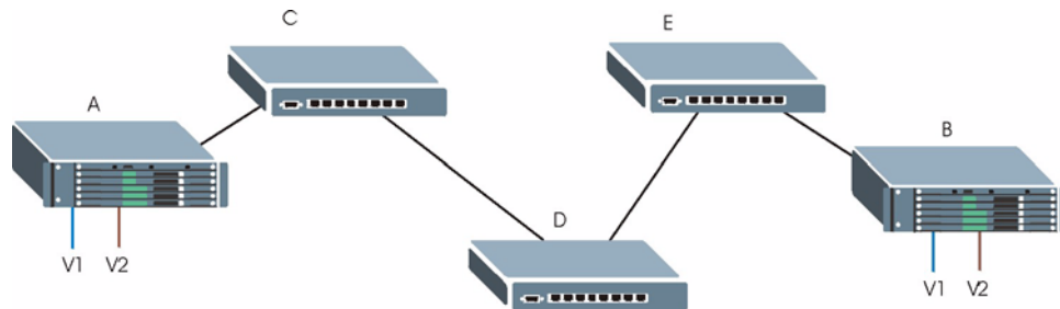
Figure 37 Port VLAN Trunking
