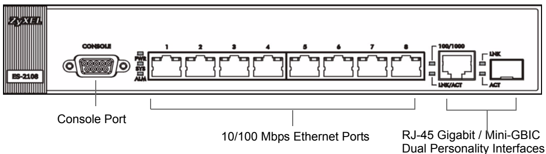
Figure 11 Front Panel: ES-2108-G/ES-2108PWR
