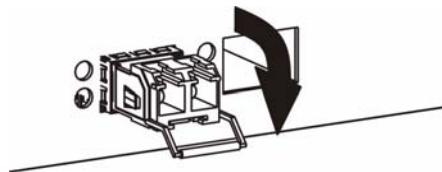
Figure 15 Opening the Transceiver's Latch Example
