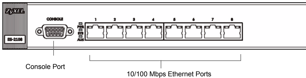
Figure 10 Front Panel: ES-2108-F
