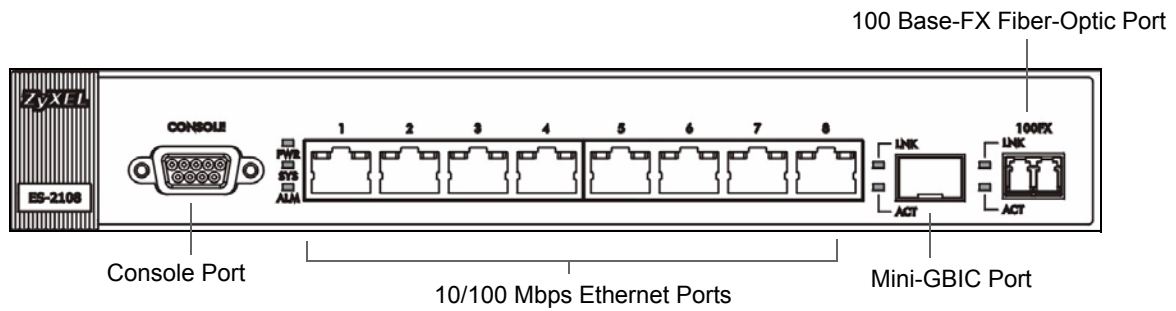
Figure 12 Front Panel: ES-2108-LC
