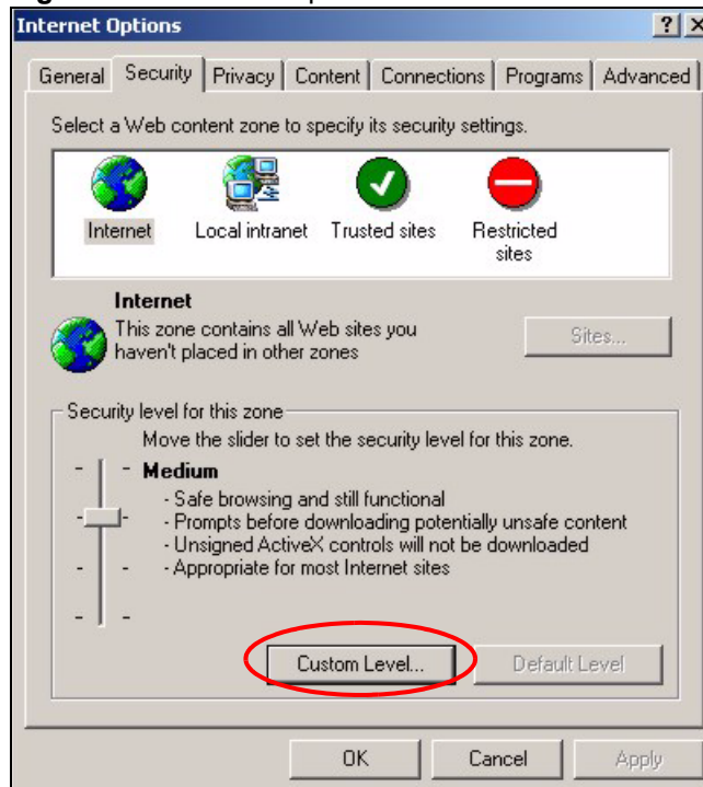
Figure 113 Internet Options
