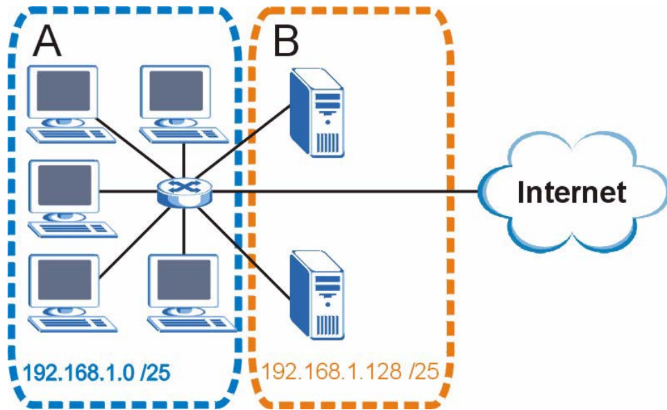
Figure 119 Subnetting Example: After Subnetting
