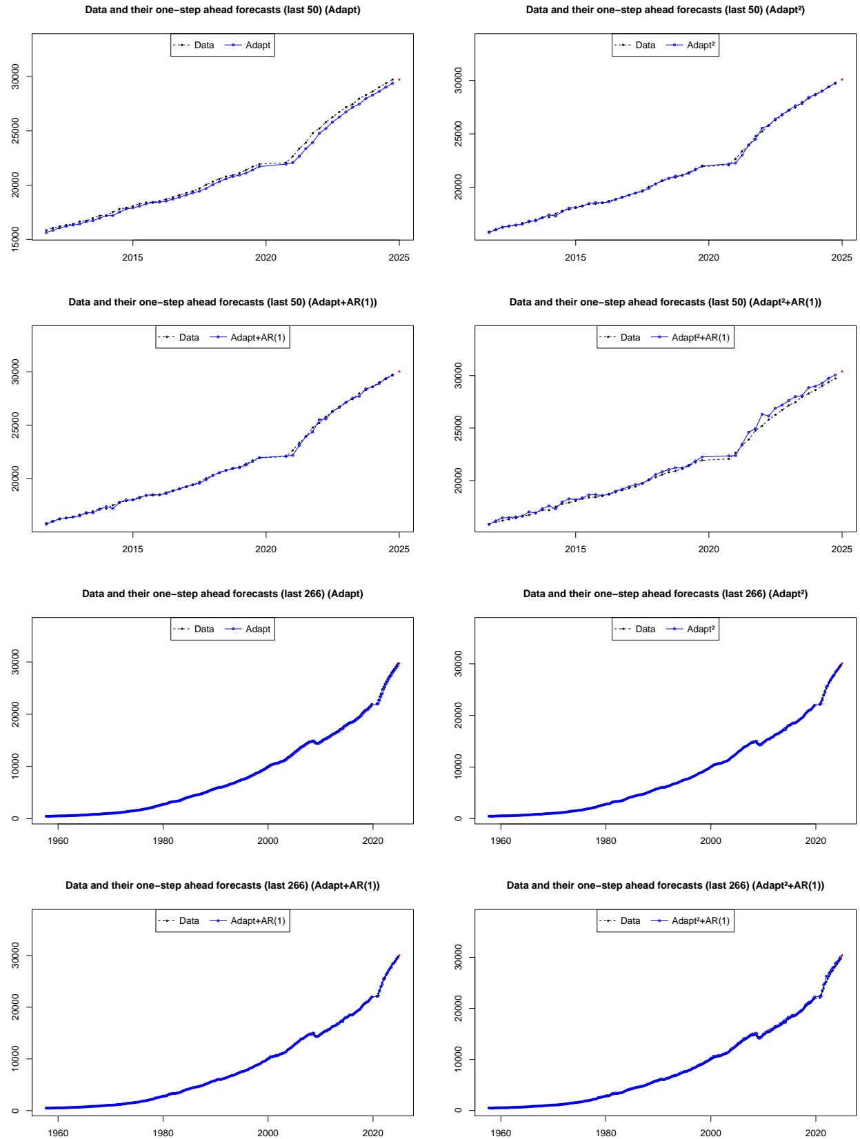
Figure 32: Data and their forecasts for the forecasting methods \text{Adapt} , \text{Adapt}+\text{AR}(1) , \text{Adapt}^2 , \text{Adapt}^2+\text{AR}(1) .
