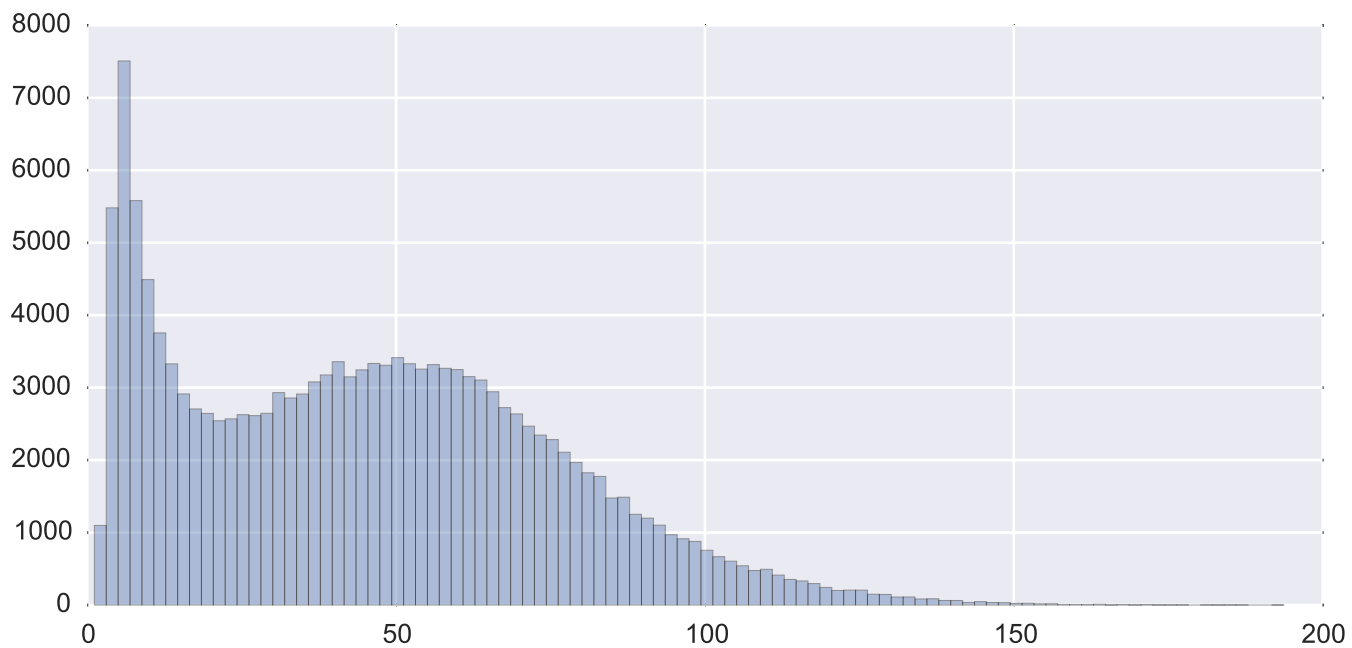
Subject 27913 tSNR inside the mask
